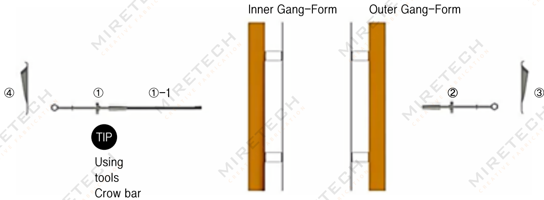
Assembly drawing
